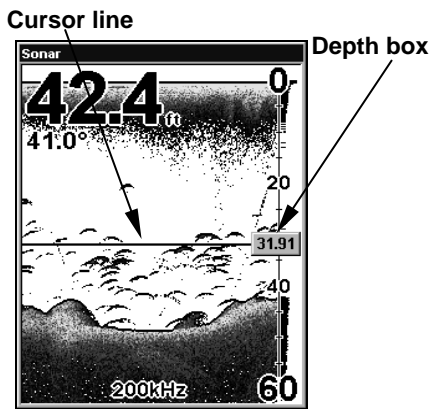
Sonar Page menu (left) with Depth Cursor command selected. Sonar chart (right) with the depth cursor active. The school of fish is 31.91 feet deep.
